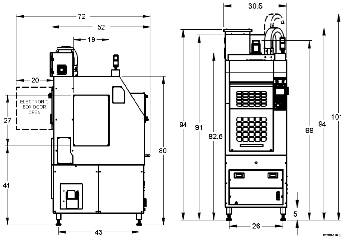
Figure 1 – Overall Dimensions of 2 OP M11
